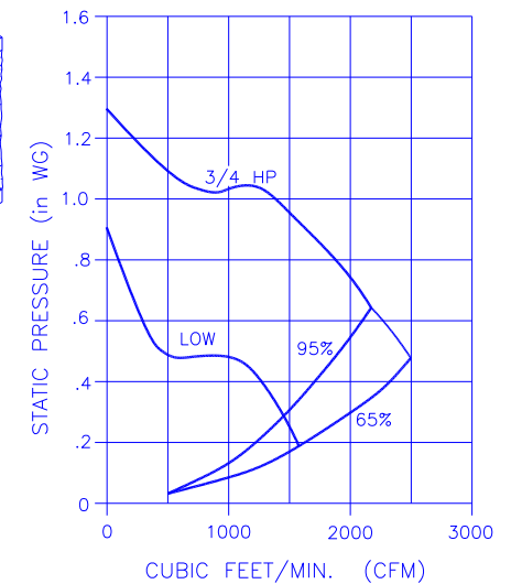
PERFORMANCE CURVES
