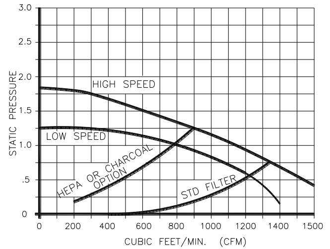
PERFORMANCE CURVES
