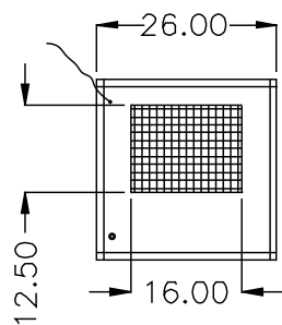
OUTLET VIEW
